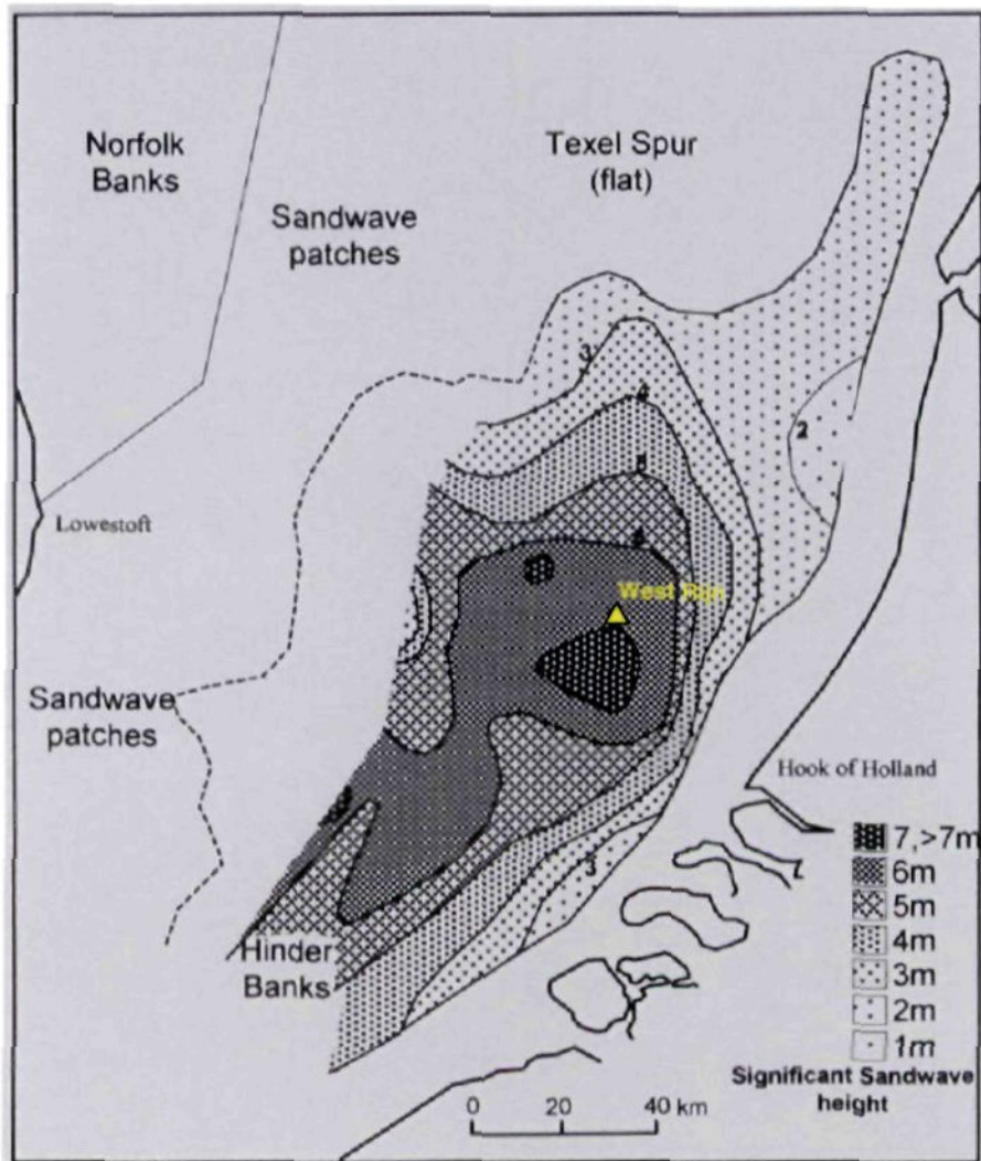
Figuur 11.6 Significant sandwave height
