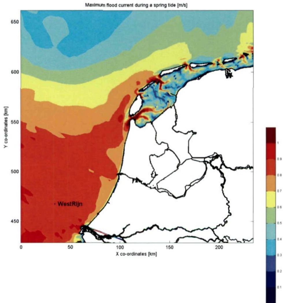
Figuur 11.2 Maximum flood current
