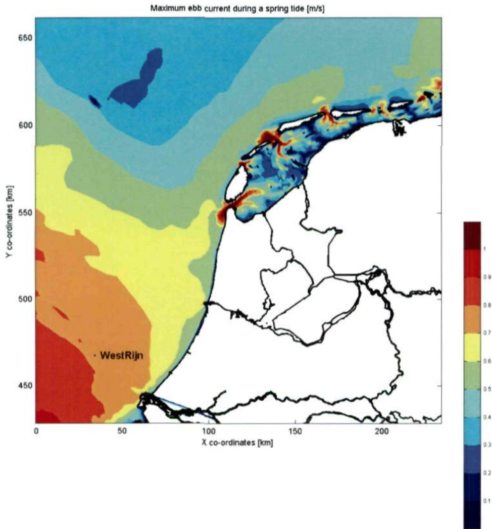
Figuur 11.3 Maximum ebb current
