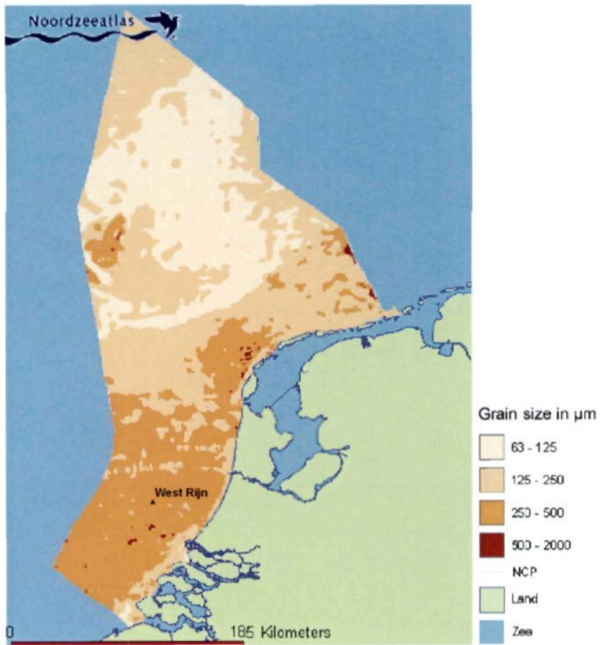
Figuur 11.5 Grain size distribution seabed surface
