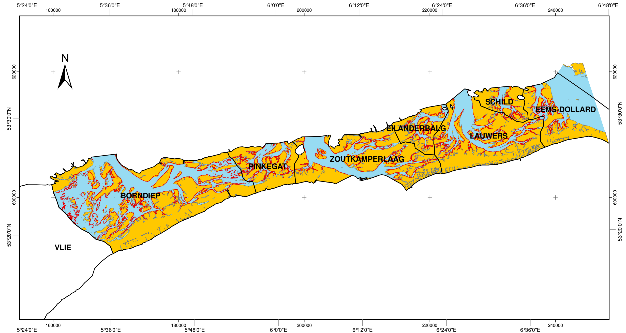
-100 cm contour of the Eastern part of the Waddensea i.r.t. 2008 aerial photograph data
