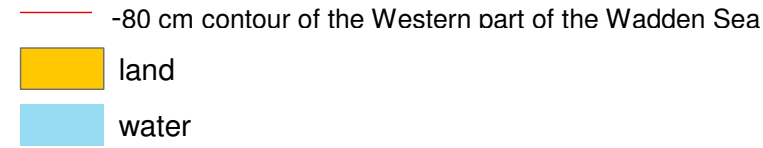
-80 cm contour of the Western part of the Waddensea i.r.t 2008 aerial photograph data
