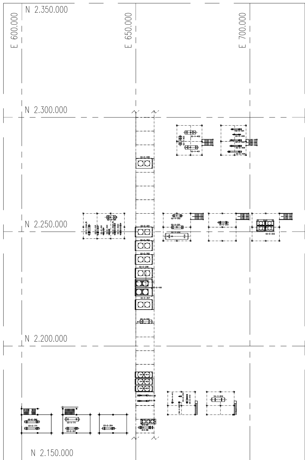
DETAIL "A" ELEVATED STRUCTURES PIPERACK (FOR REFERENCE)
